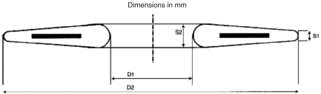
Example for Gasket dimensions Type G-S-Standard
